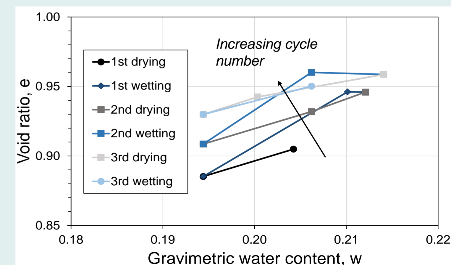
Figure 6- Cyclic drying and wetting SCs (Y3)
