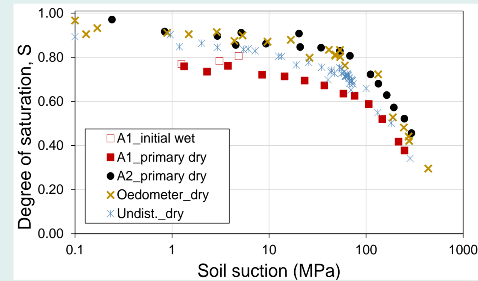
Figure 1- Drying curves for A1 & A2
