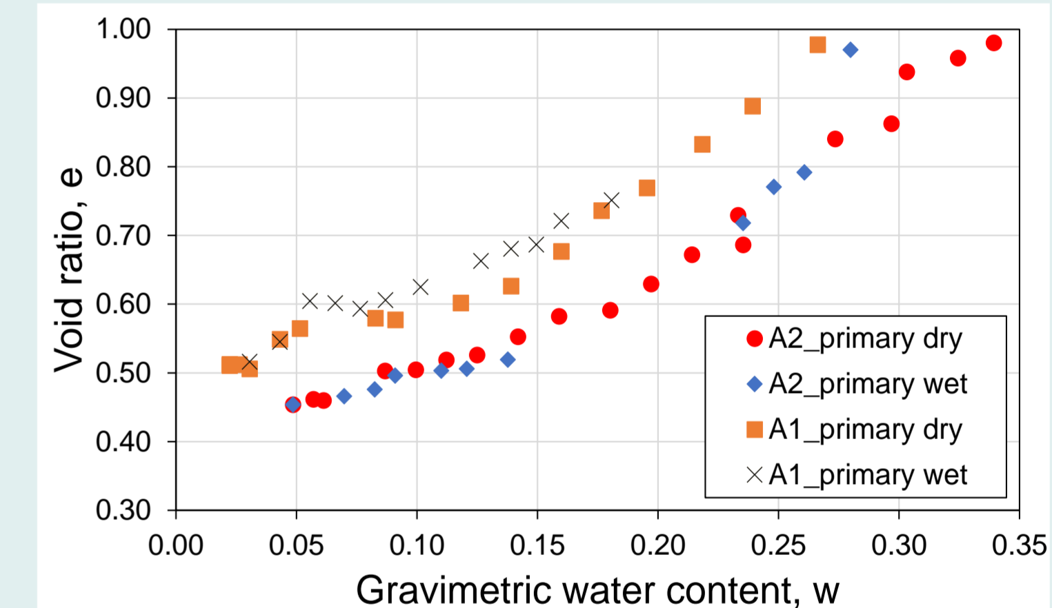
Figure 4- Drying and wetting SCs (A1 & A2)
