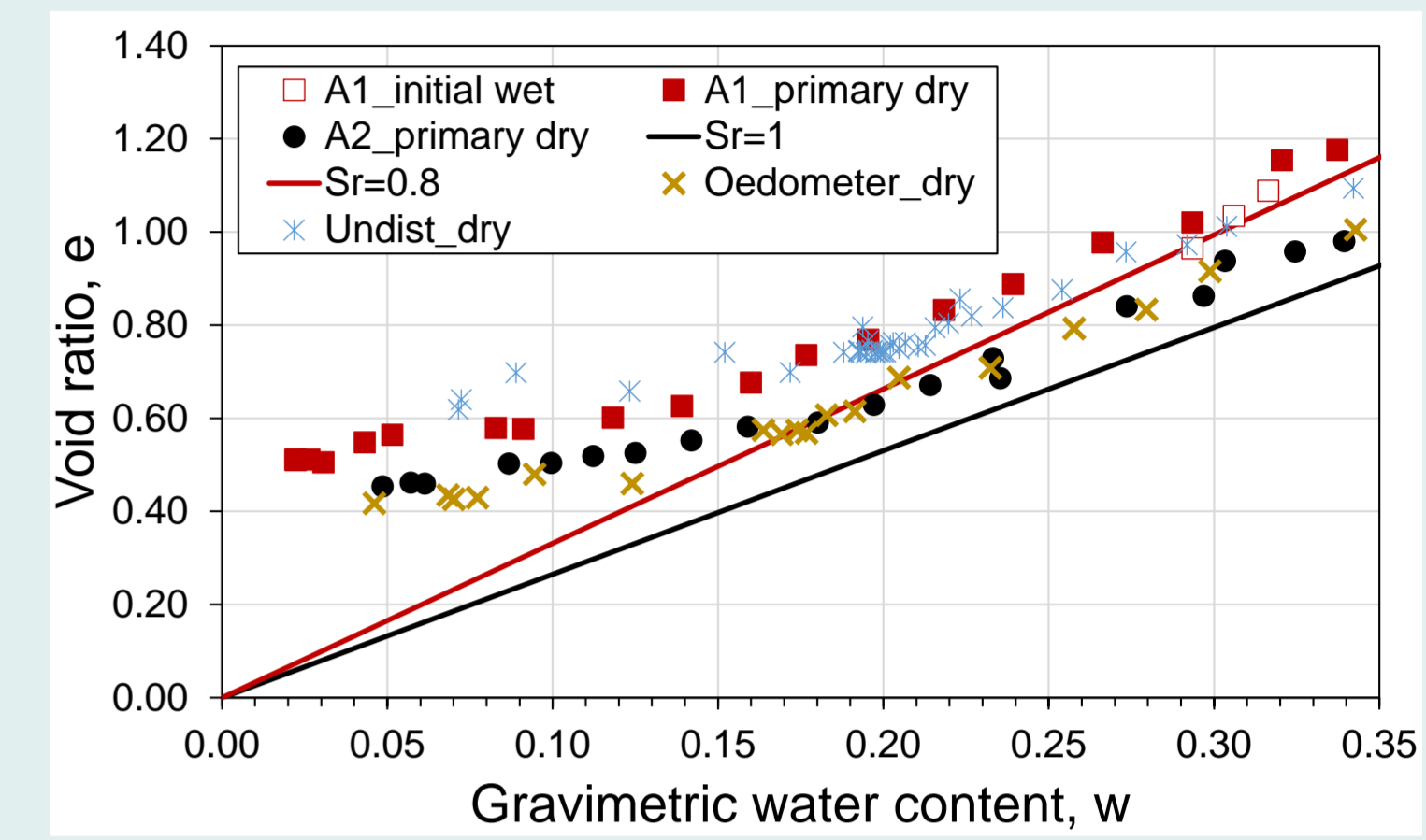
Figure 2- Drying SCs (A1 & A2)
