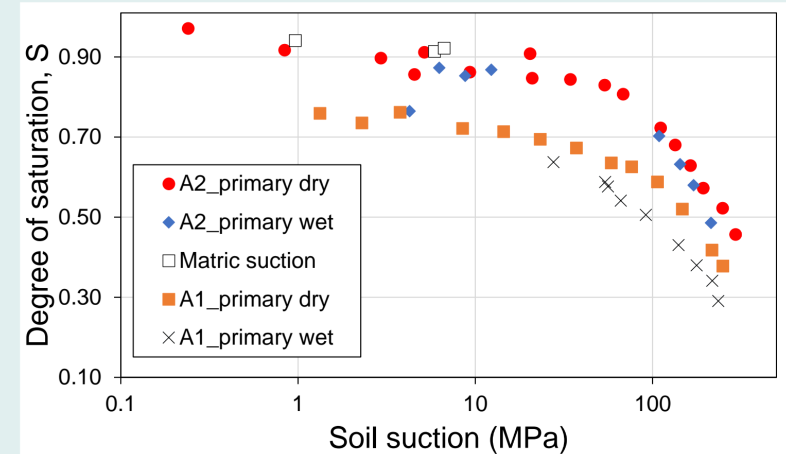
Figure 3- Drying and wetting curves (A1 & A2)
