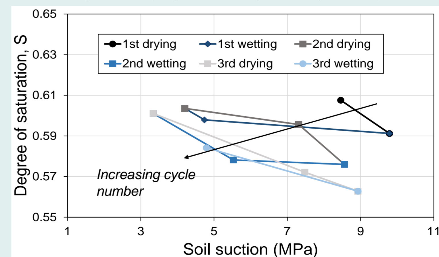
Figure 5- Cyclic drying and wetting curves for Y3
